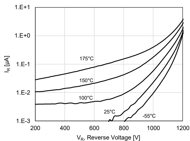
Figure 4. Reverse Characteristics
