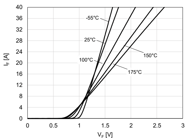
Figure 3. Forward Characteristics
