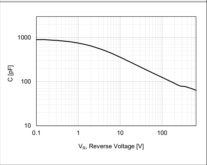
Figure 7. Capacitance Characteristic
