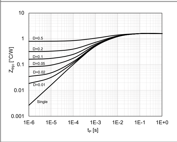
Figure 8. Transient Thermal Response Curve
